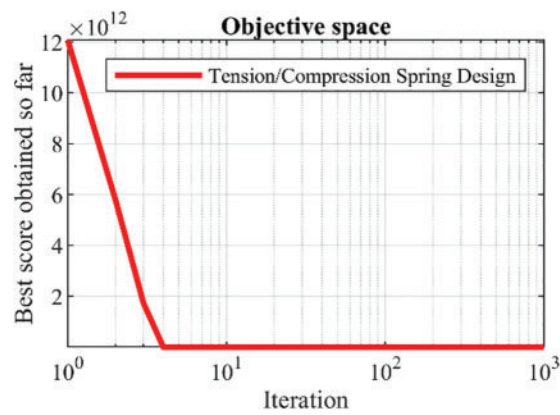
Figure 20: FNO's performance convergence curve on tension/compression spring
